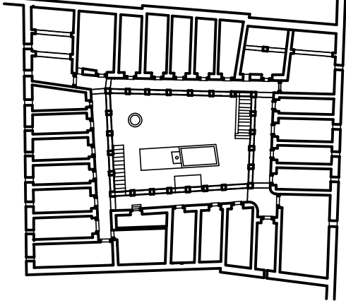
plan R+1 Ech: 1/200
